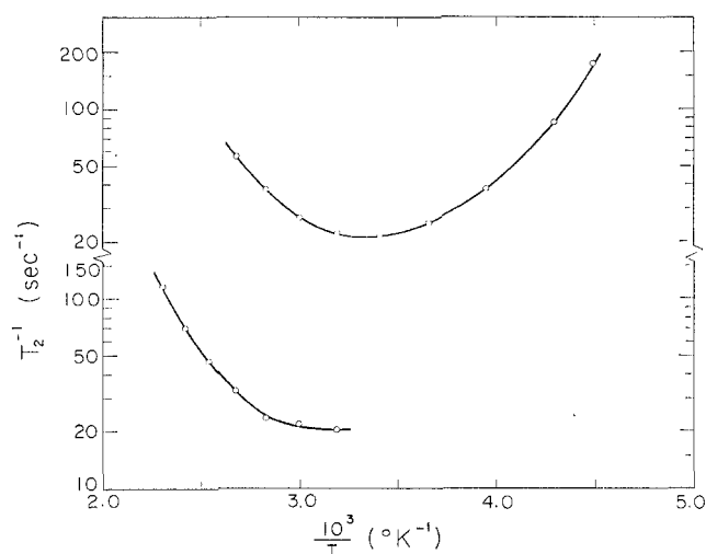
Figure 2.—The temperature dependence of \log(T_2^{-1}) for an \text{HSO}_3\text{Cl} solution (upper curve) of \text{Co}(\text{NH}_3)_5\text{SO}_3\text{Cl}^{2+} and for a concentrated \text{H}_2\text{SO}_4 solution (lower curve) of \text{Co}(\text{NH}_3)_5\text{HSO}_4^{2+} .
