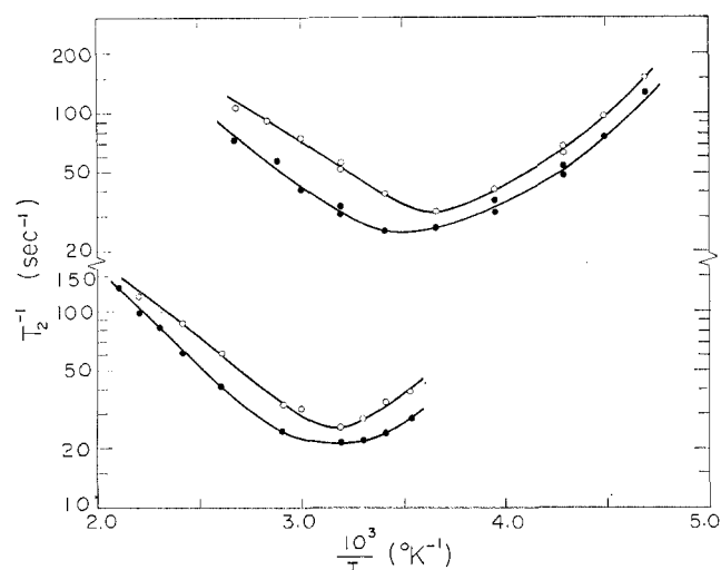
Figure 1.—The temperature dependence of \log(T_2^{-1}) for solutions of \text{Co}(\text{NH}_3)_6^{3+} and \text{Rh}(\text{NH}_3)_6^{3+} in \text{HSO}_3\text{Cl} (upper curves) and concentrated \text{H}_2\text{SO}_4 (lower curves). The symbols ● and ○ refer to \text{Rh}(\text{NH}_3)_6^{3+} and \text{Co}(\text{NH}_3)_6^{3+} , respectively.
