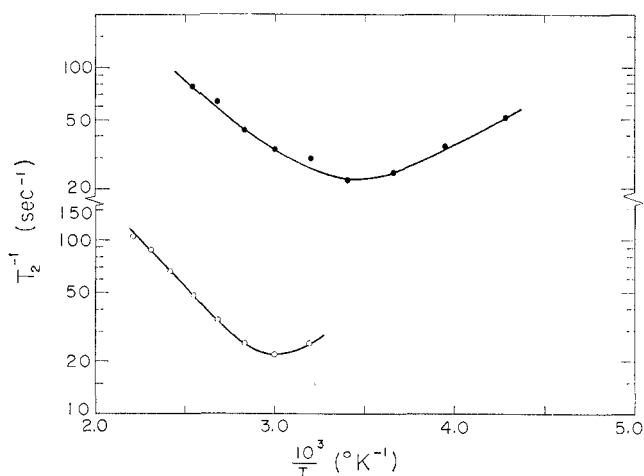
Figure 3.—The temperature dependence of \log(T_2^{-1}) for an \text{HSO}_3\text{Cl} solution (upper curve) of \text{Rh}(\text{NH}_3)_5\text{SO}_3\text{Cl}^{2+} and for a concentrated \text{H}_2\text{SO}_4 solution (lower curve) of \text{Ir}(\text{NH}_3)_5\text{HSO}_4^{2+} .
